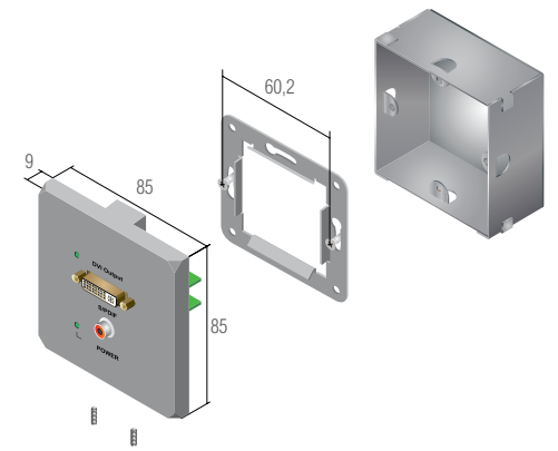
Dismounted diagram Dimensions shown in millimeters.
